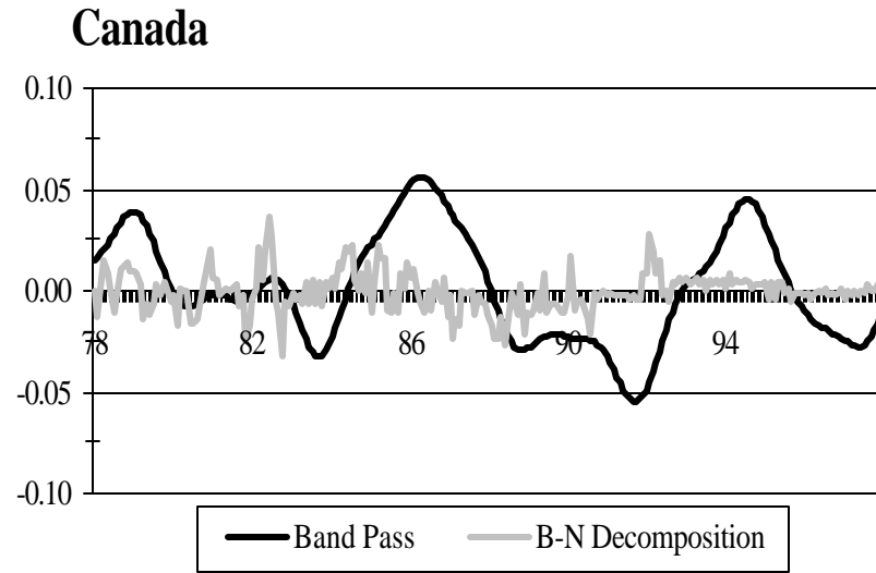
Figure 1: Temporary Components of Spot Rates
